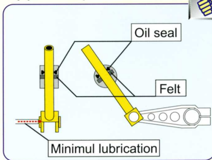
Upper looper
