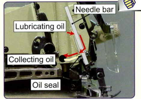
Needle bar
